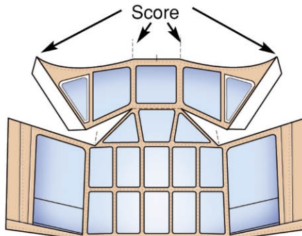
Cockpit Canopy
